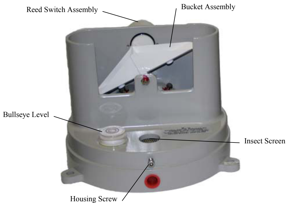
FIGURE 7-1. Components of CS700 Base
