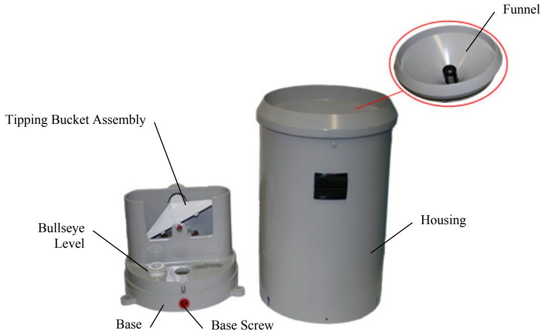
FIGURE 3-4. Main Components of the CS700
