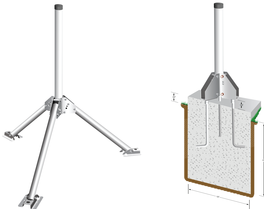
FIGURE 3-3. Pedestal Base Options
