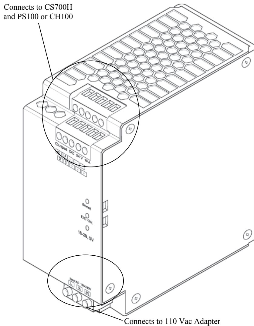
FIGURE 4-2. Phoenix Contact Power Supply
