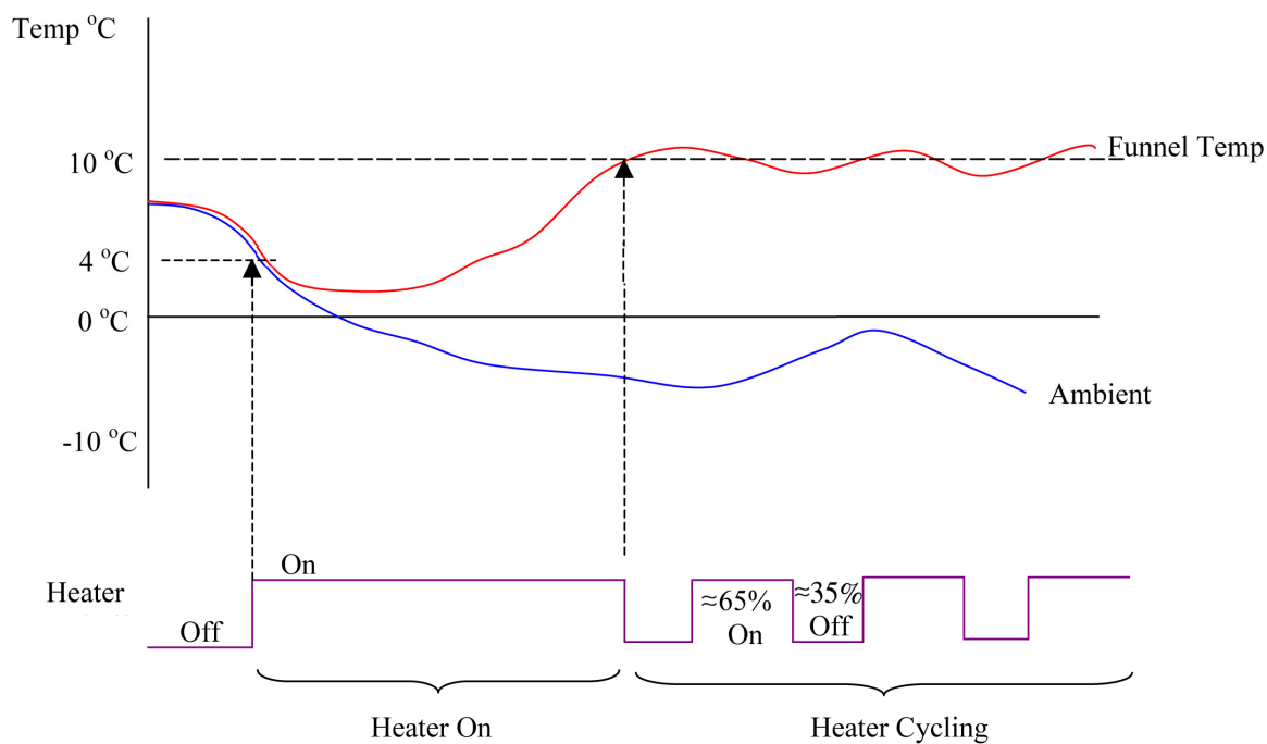
FIGURE 2-1. Heater Operation
