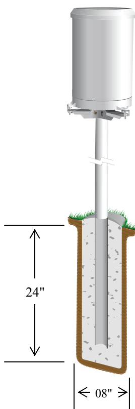
FIGURE 3-2. Typical Rain Gage Installation
